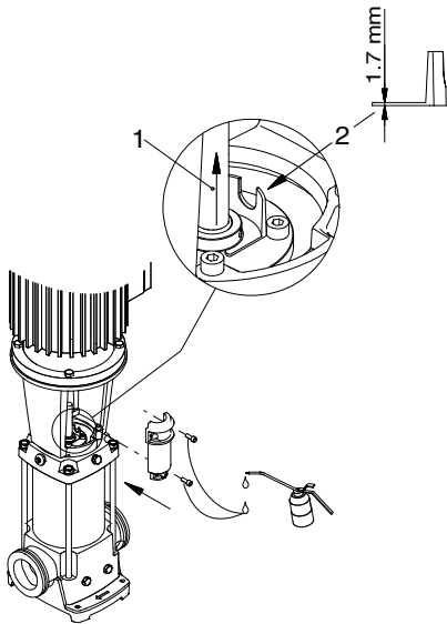
Рис. 8 CR, CRN 32, 45, 64, 90
