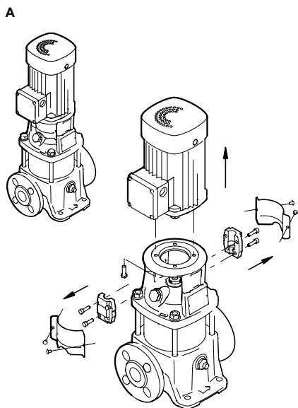
Рис. 7 CR, CRI, CRN 10, 15 and 20
